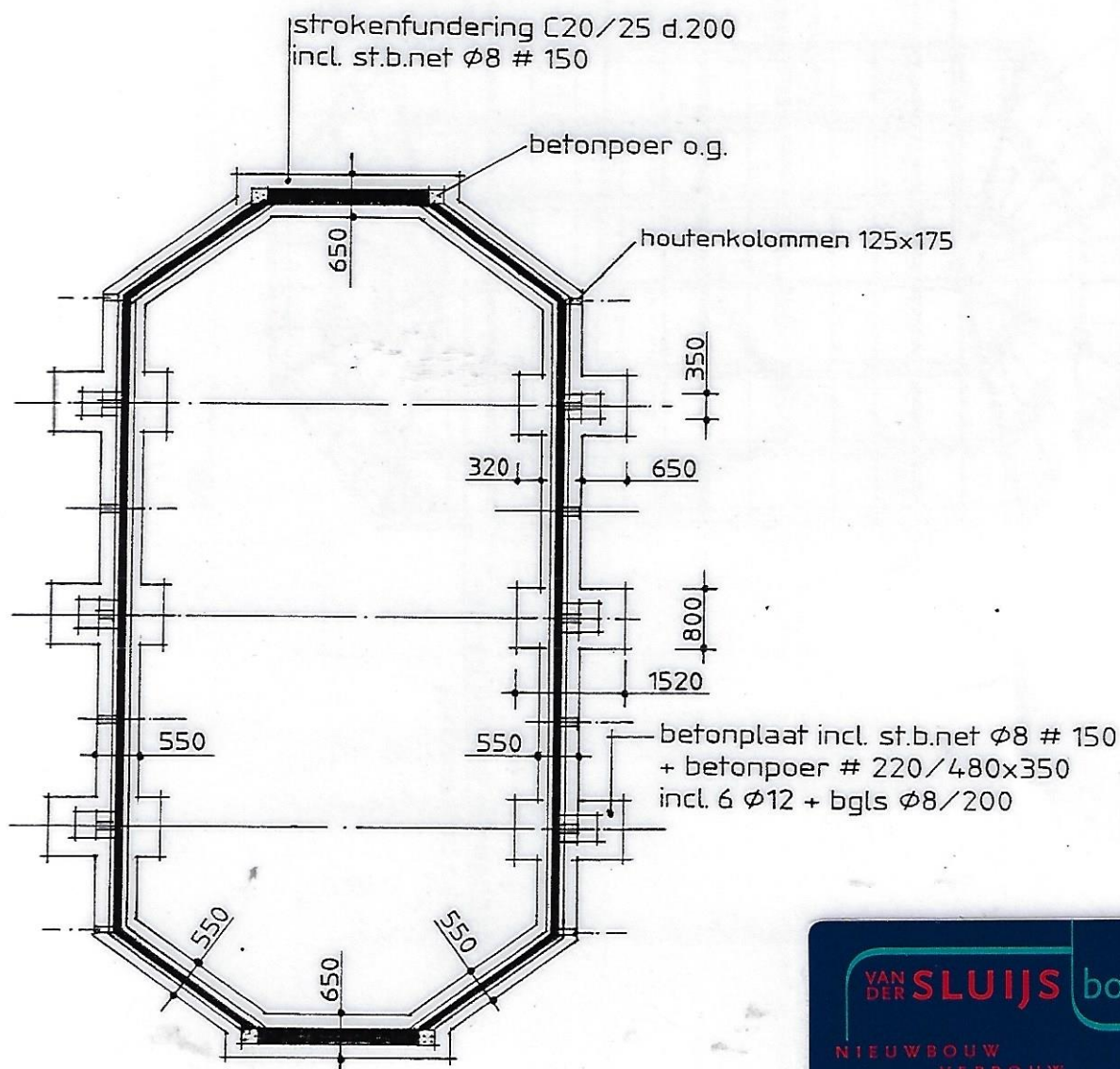
funderingsplan
