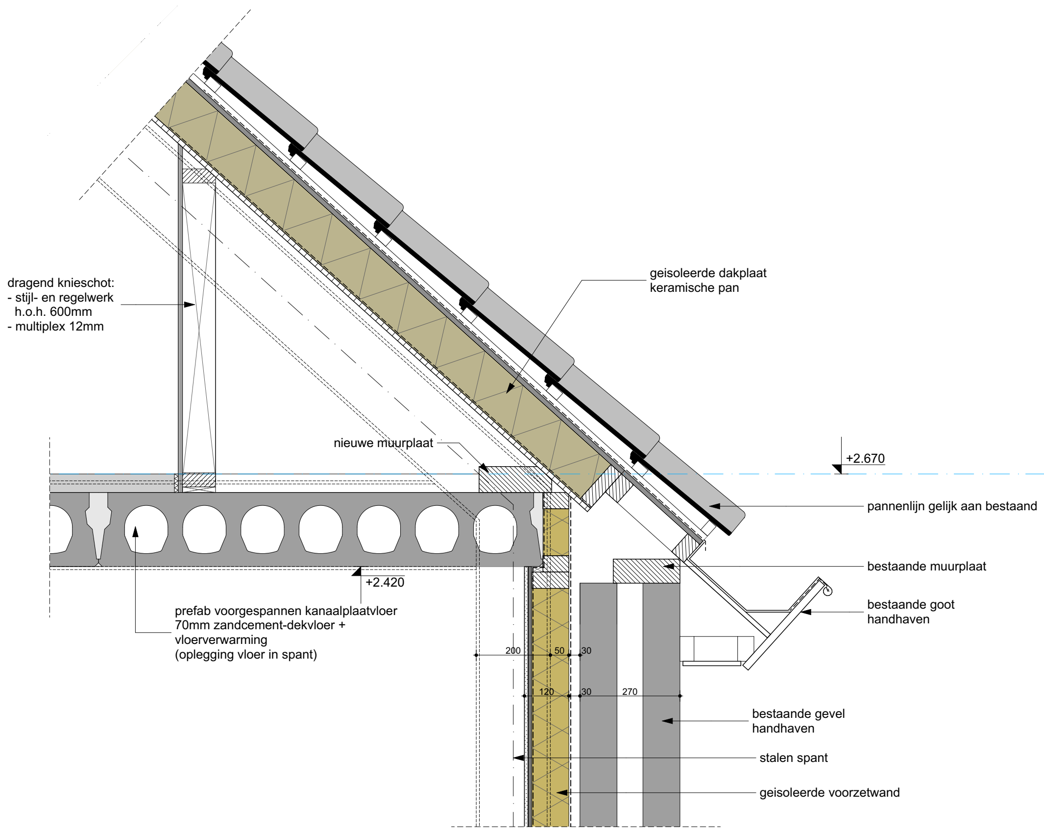
PRINCIPE DETAIL TPV GOOT schaal 1:10
