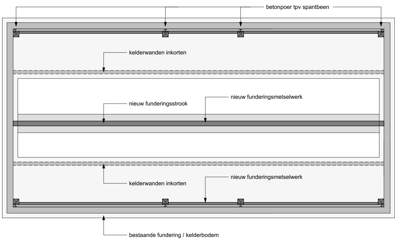
SCHEMA FUNDERING
