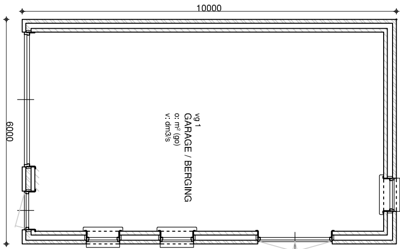
BEGANE GROND GARAGE
