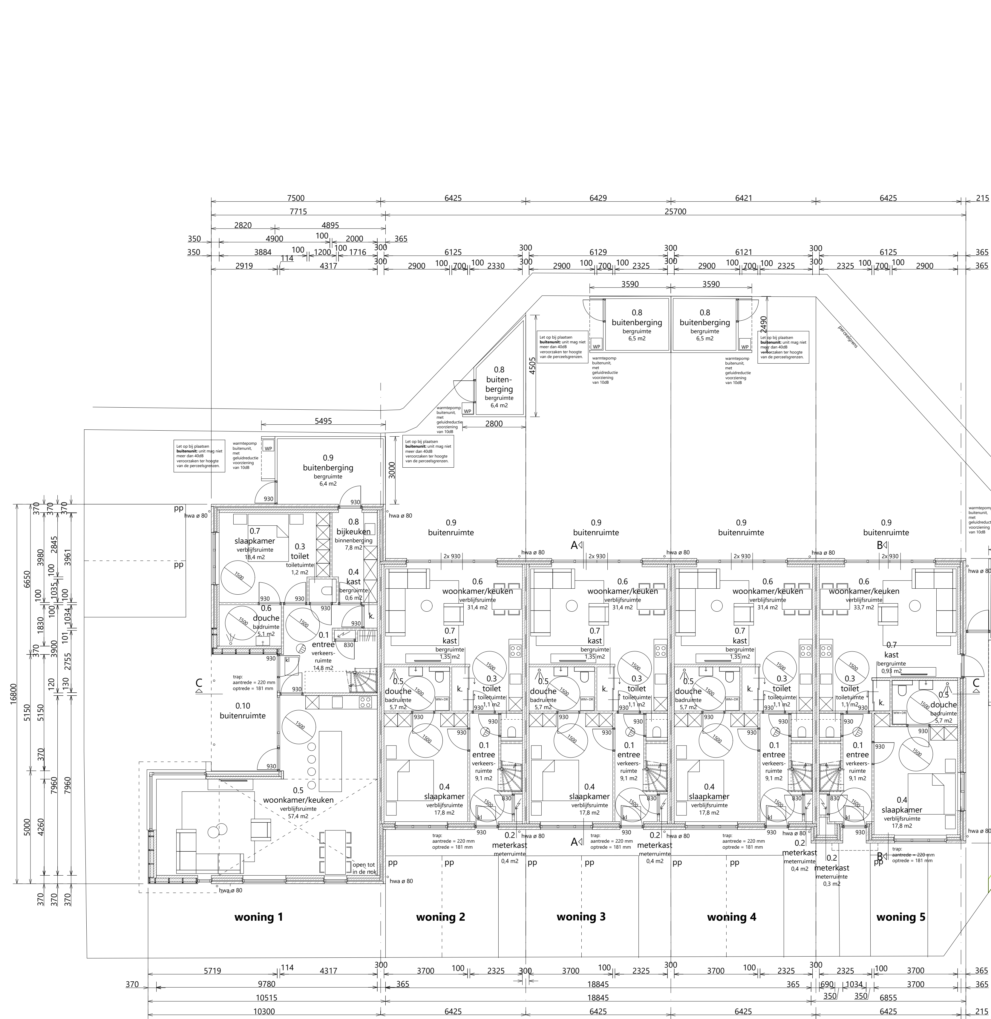
beganeggrond
