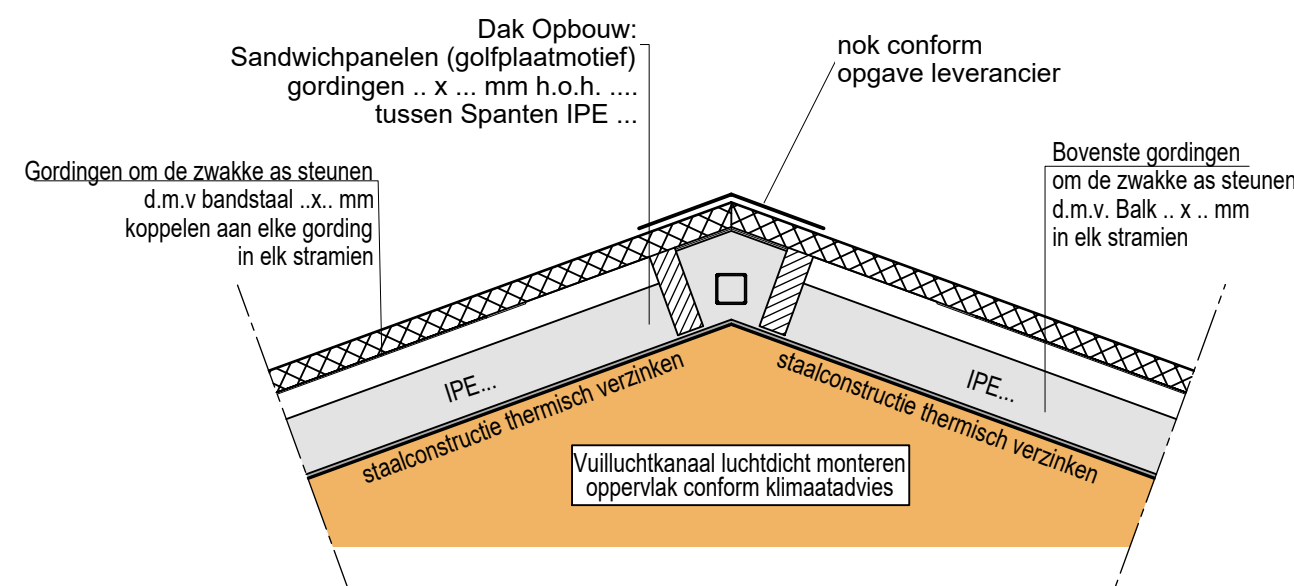
3. Principe detail nok
