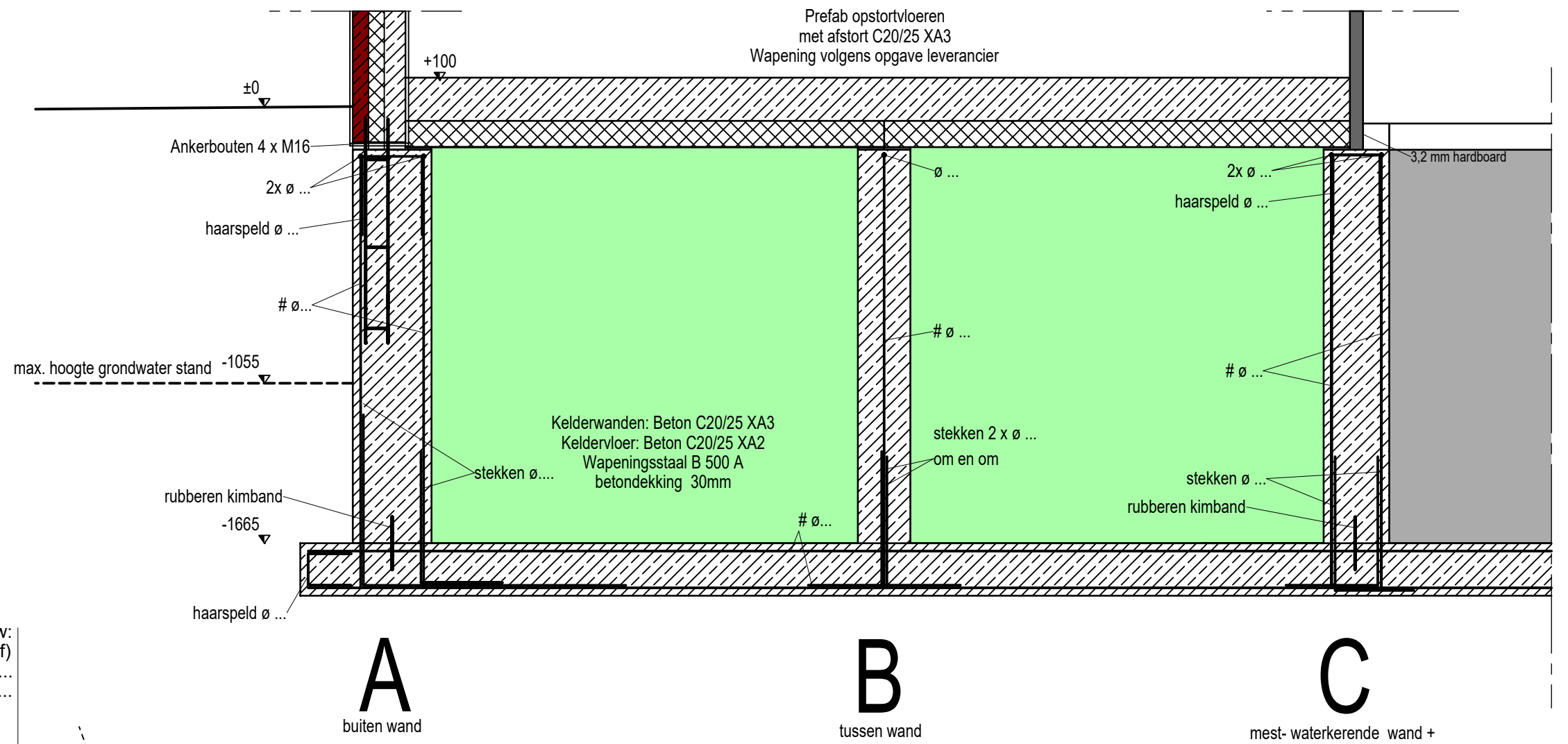
1. Principe detail kelderwanden
