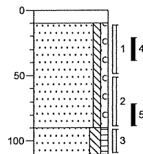
Boring: A04
