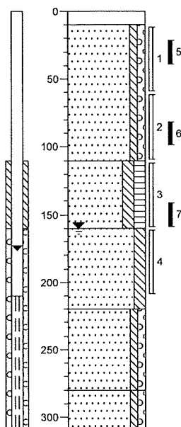
Boring: A01
