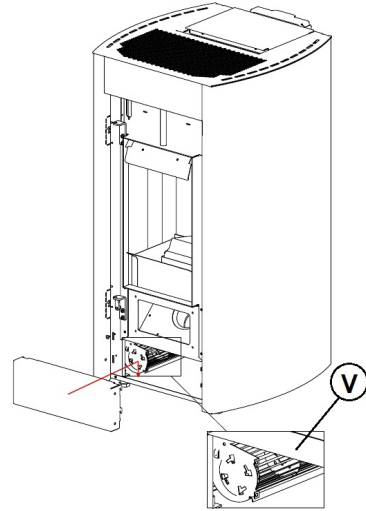
Fig. 71 - Ventilators
