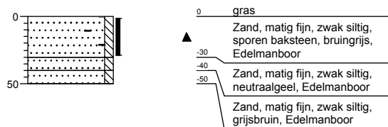
boring 6
