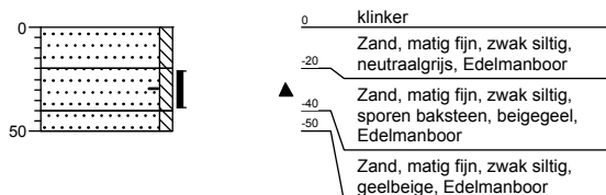
boring 13
