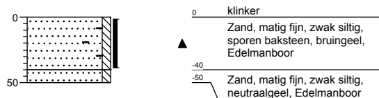
boring 14
