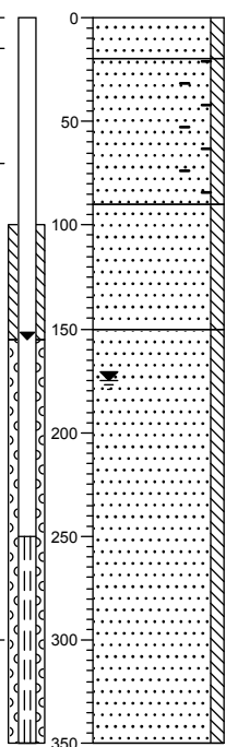
boring 2
