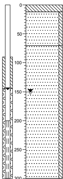
boring 1
