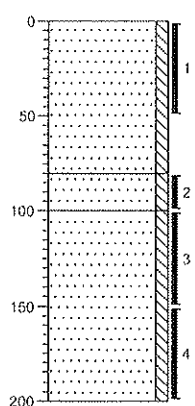
boring 5
