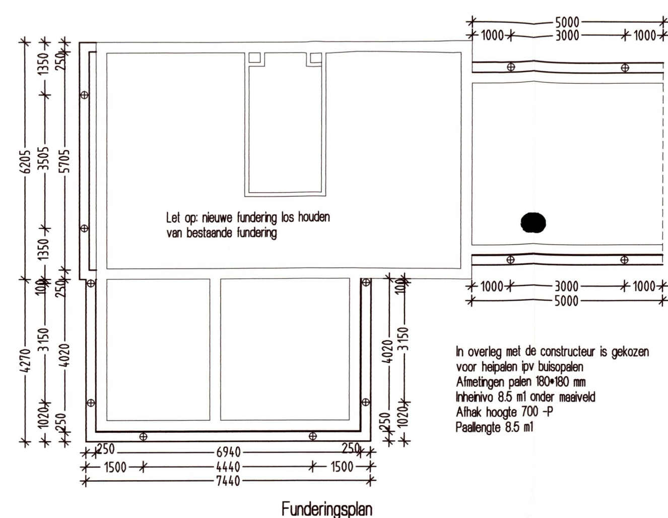
Funderingsplan
