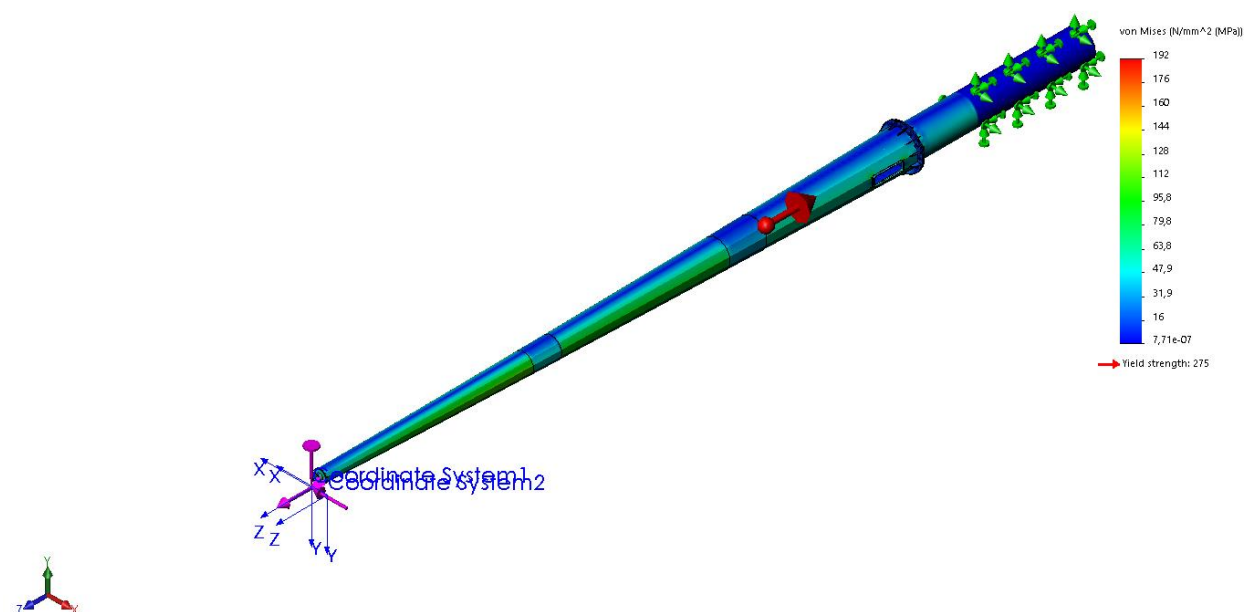
Mast 20mtr REV2 Assembly-Static 1-Stress-Stress1
