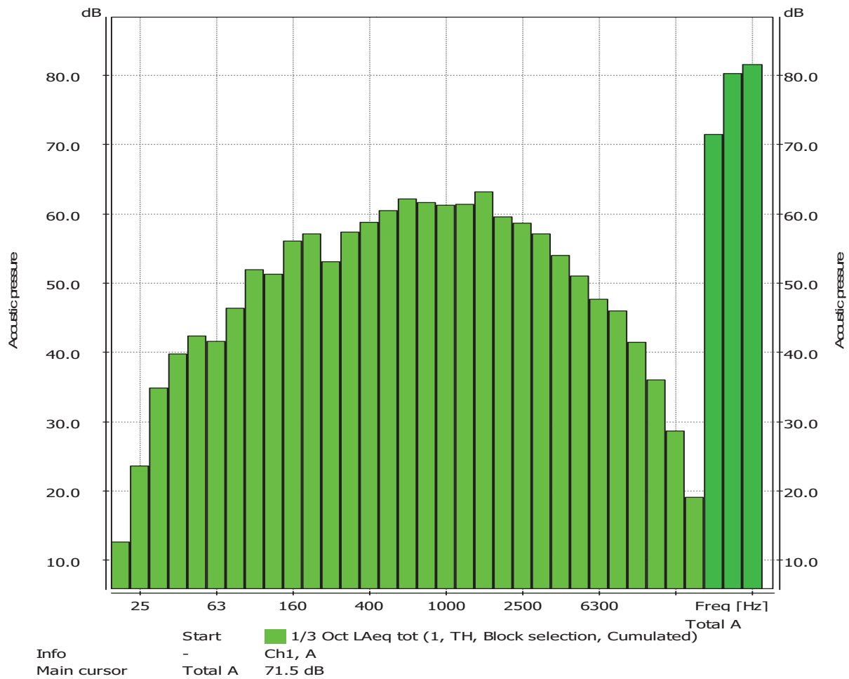
Logger 1/3 Octave, 11-11-2016 14:01:35.000
