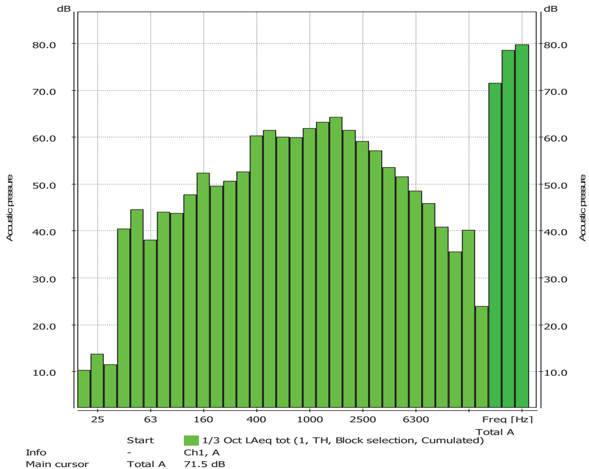
Logger 1/3 Octave, 11-11-2016 13:55:48.300
