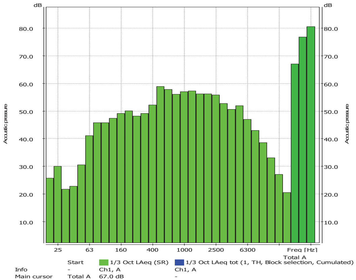
Logger 1/3 Octave, 11-11-2016 13:50:18.500
