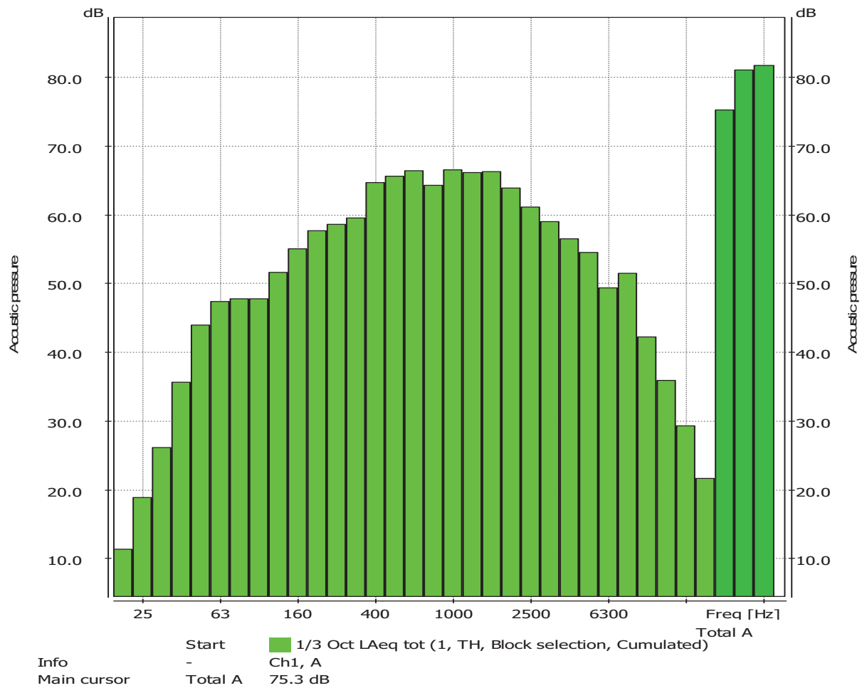
Logger 1/3 Octave, 11-11-2016 13:59:10.800
