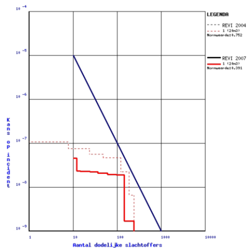
Figuur 10: Groepsrisicocurve LPG-tankstion BIM
